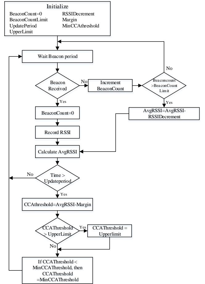
Fig. 2: Flow chart of DSC algorithm used at each non-AP station.
